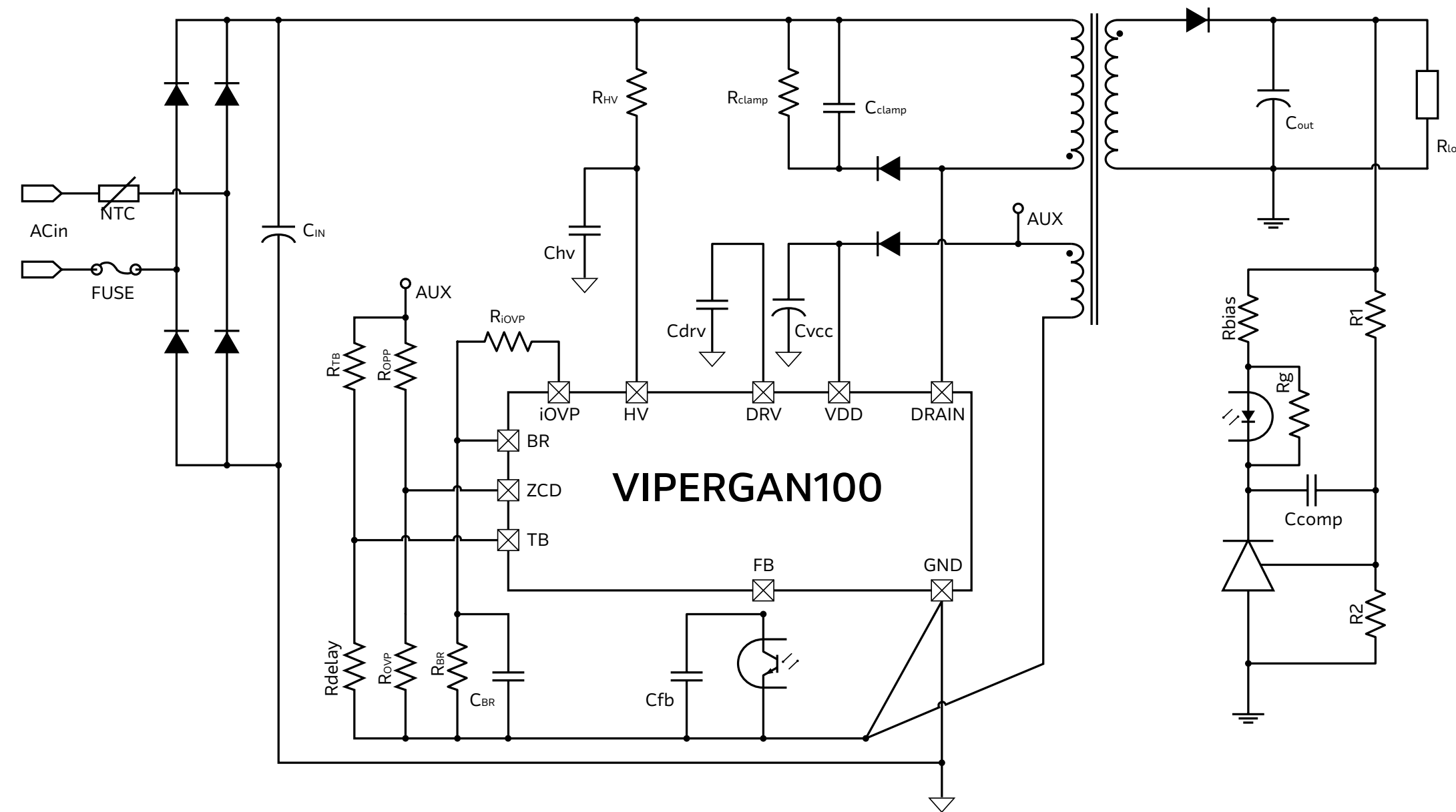
Example circuit for a VIPERGAN100
