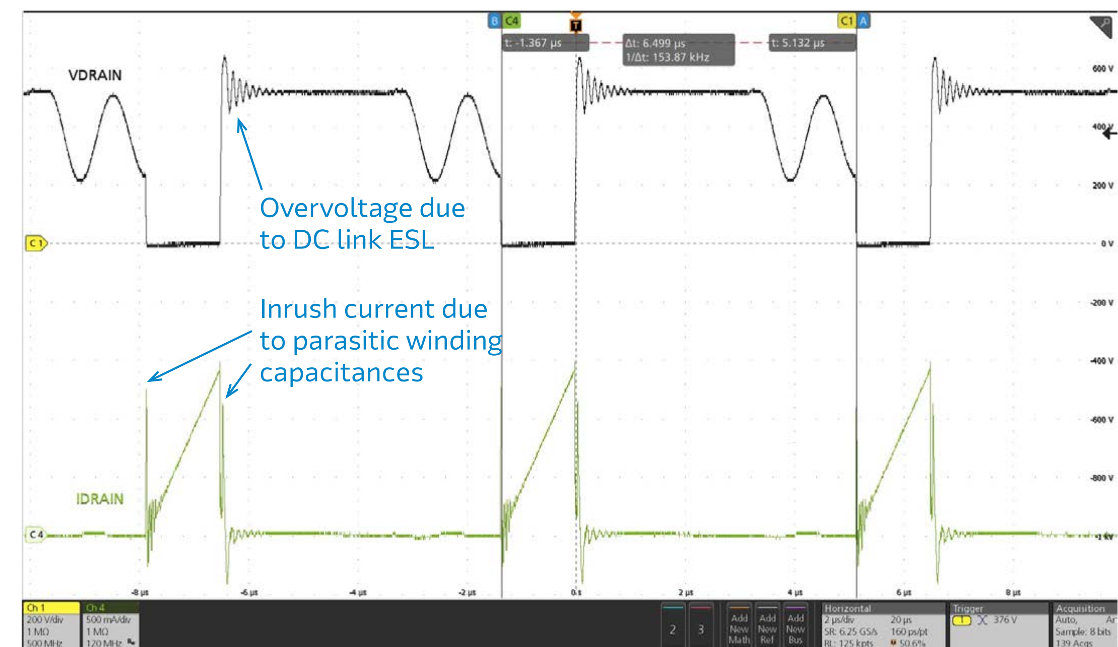
Figure 2: STMicroelectronics, EVLVIPGAN50FL: 15 V / 50 W isolated flyback with VIPERGAN50, Application note AN5844, Rev. 2, June 2024, STMicroelectronics. Available: st.com/resource/en/application_note/an5844-evlvipgan50fl-15-v50-w-isolated-flyback-with-vipergan50-stmicroelectronics.pdf
