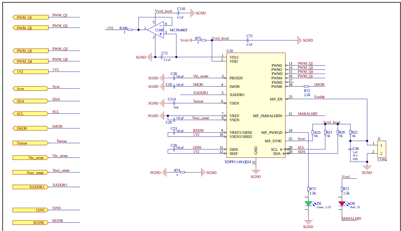
Figure 8 Control schematic
