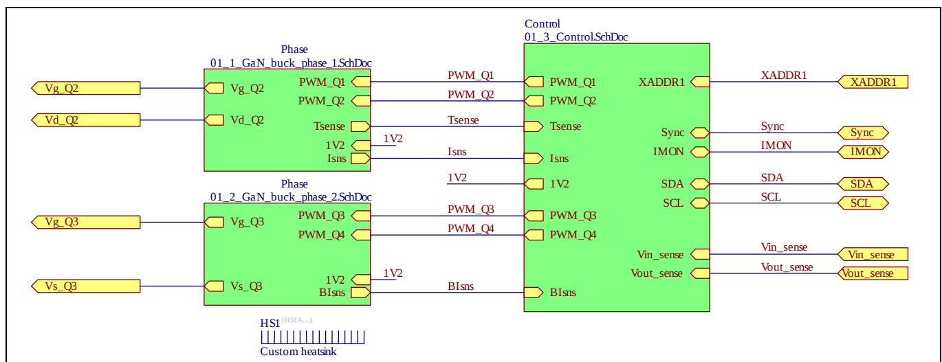
Figure 5 Power stage schematic (top hierarchy)
