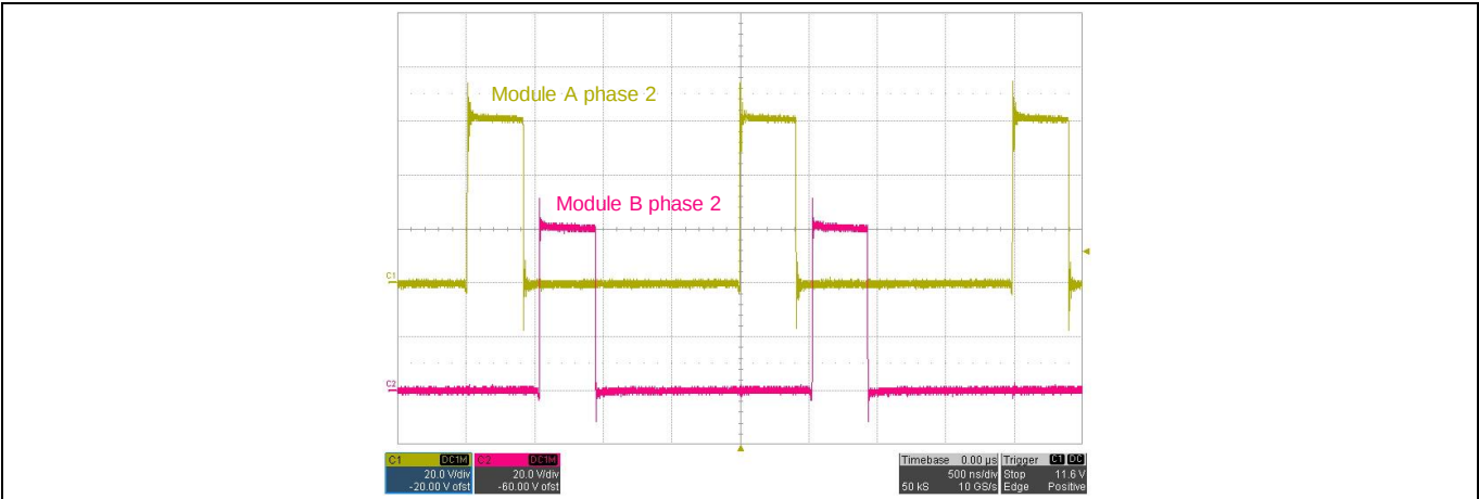
Figure 16 Switching node waveforms: 60 Vin, 12 Vout, 134 A out
