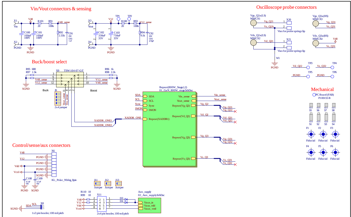
Figure 4 Main schematic
