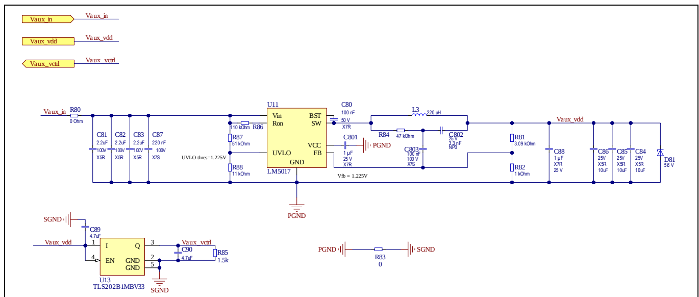
Figure 9 Housekeeping power supplies schematic
