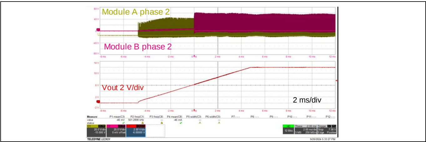
Figure 17 Start-up waveforms: 48 Vin, 12 Vout, 0 A out
