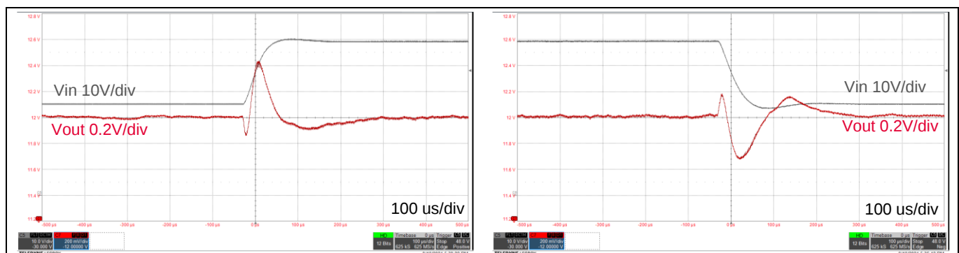
Figure 19 Line transient response: 36 V in to 60 V in and 60 V in to 36 V in , 12 V out , 20 A output, 0.3 V/μs slew rate
