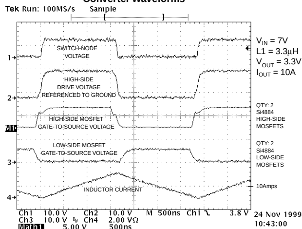
Converter Waveforms
