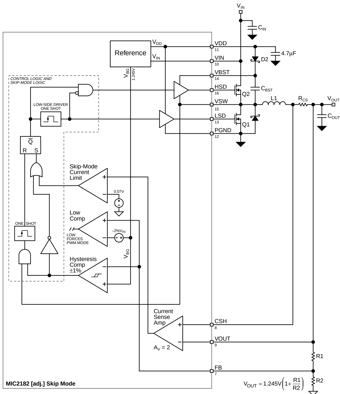
Figure 4. Skip-Mode Operation
