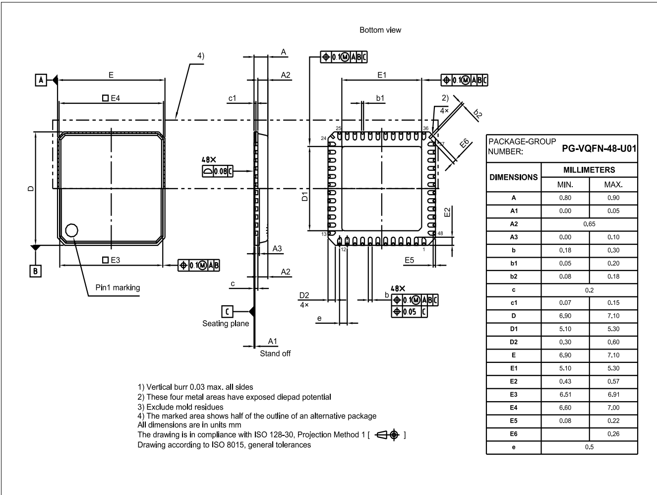
Figure 69 PG-VQFN-48 1)
