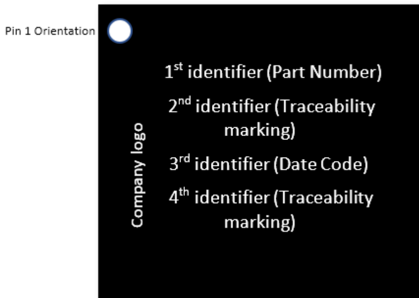
Figure 2. 249-pin FOWLP package markings
