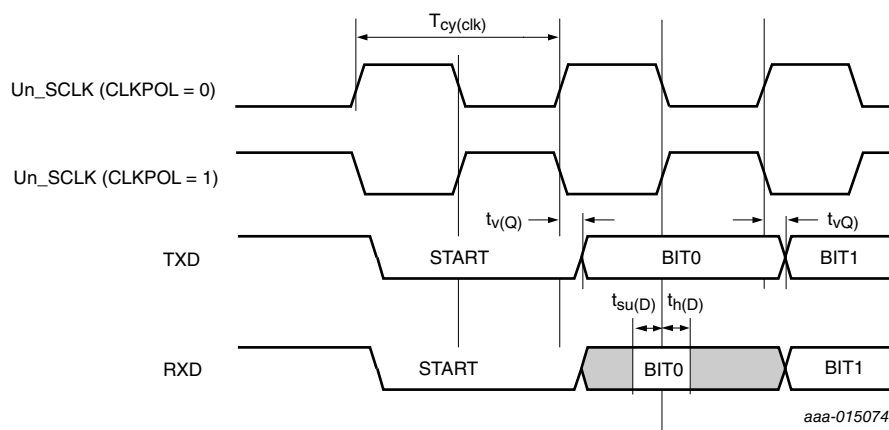
Figure 24. USART timing
