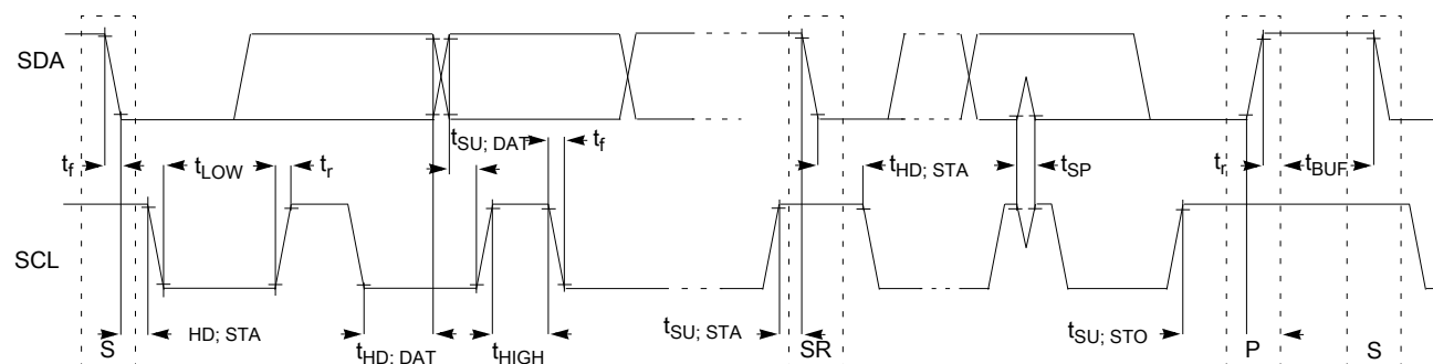
Figure 34. Timing definition for devices on the I2C bus
