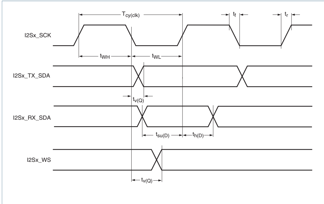
Figure 26. I 2 S-bus timing (master)
